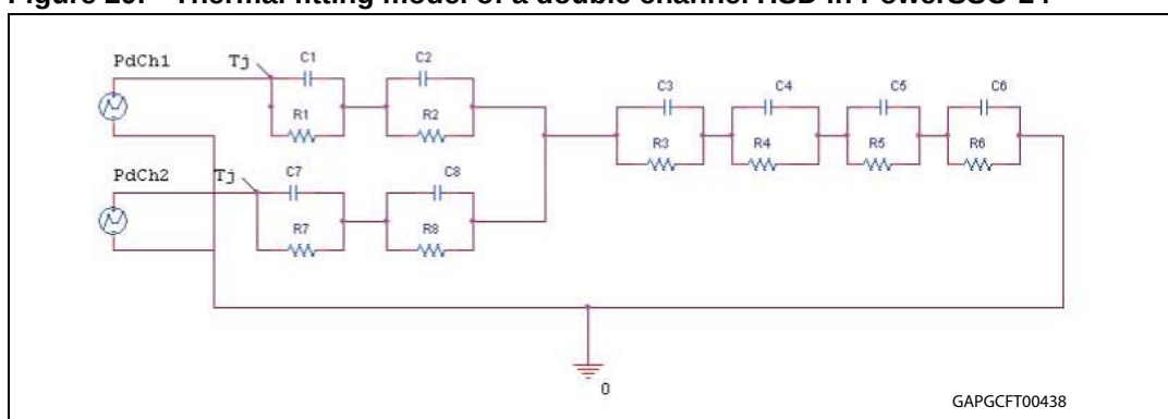
Figure 29. Thermal fitting model of a double channel HSD in PowerSSO-24 (1)
