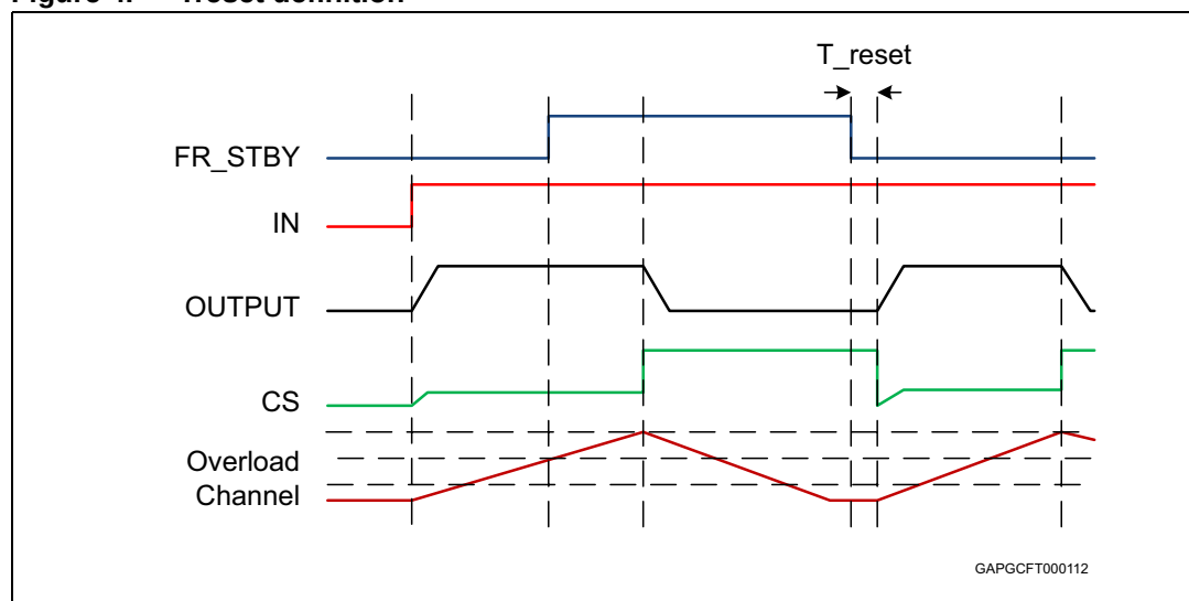
Figure 4. Treset definition
