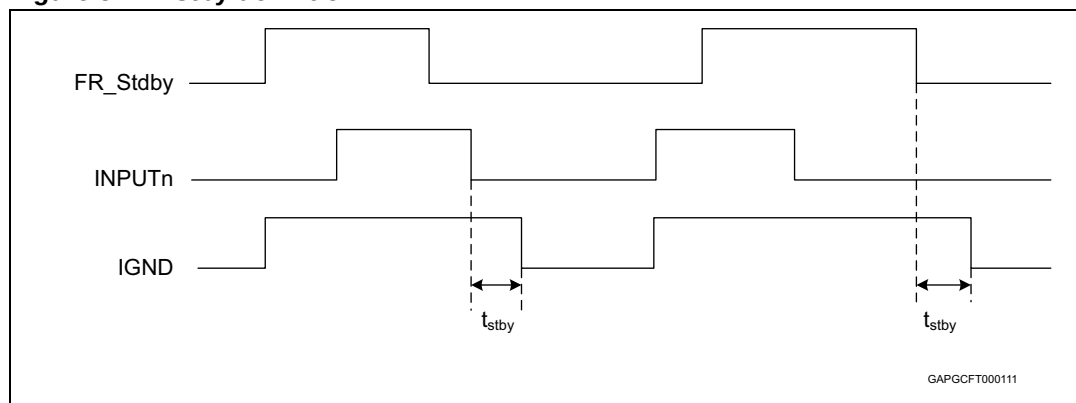
Figure 5. Tstby definition
