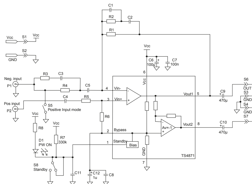
Figure 82. Demoboard schematic
