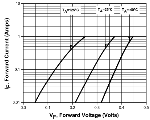
Forward Voltage for CMSH1-40ML
