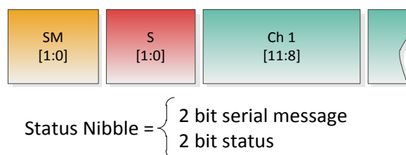
fig. 16 - SENT Status Nibble and Serial Message
