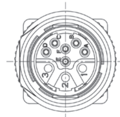
Plug, straight, panel mount, Checkmate™
