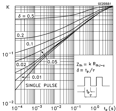
Figure 2. Thermal impedance
