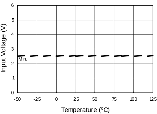
Figure 19A. Logic "1" Input Voltage vs. Temperature
