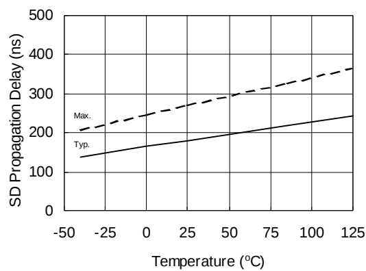
Figure 15A. SD Propagation Delay vs. Temperature
