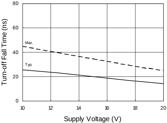
Figure 17B. Turn-Off Fall Time vs. Supply Voltage
