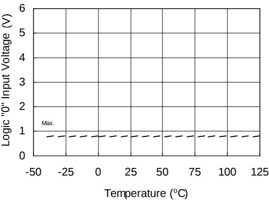
Figure 20A. Logic "0" Input Voltage vs. Temperature
