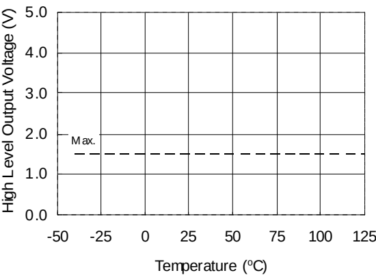
Figure 23A. High Level Output Voltage vs. Temperature ( I_O = 0 mA)
