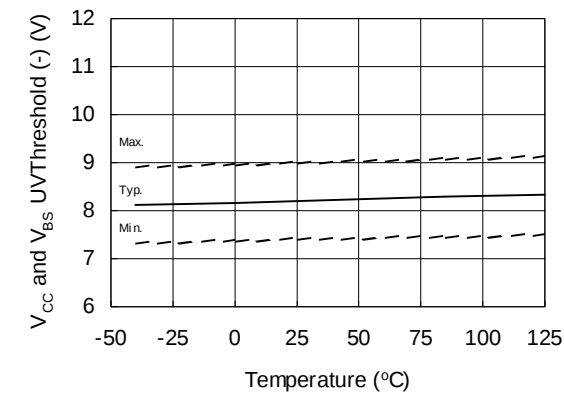
Figure 31. V_{CC} and V_{BS} Undervoltage Threshold (-) vs. Temperature
