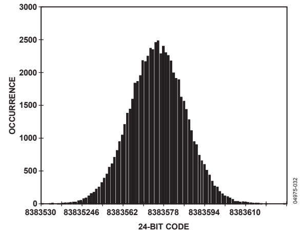
Figure 32. Low Power, 24-Bit Histogram, 256x Decimation
