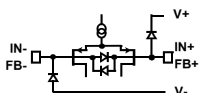
CIRCUIT 1A
