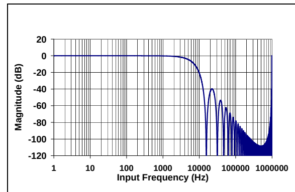
FIGURE 5-3: SINC Filter Response with MCLK = 4 MHz, OSR = 64, PRESCALE = 1.
