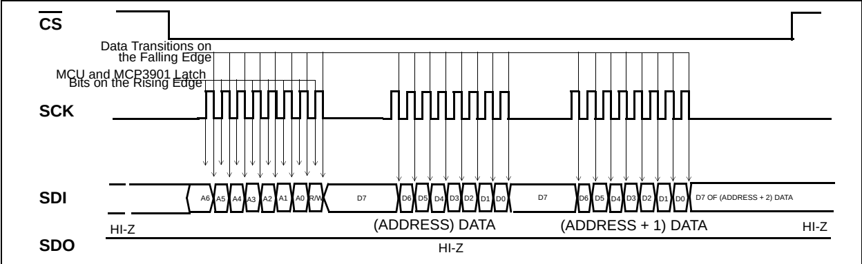
FIGURE 6-5: Device Write (SPI Mode 0,0 - Clock Idles Low).
