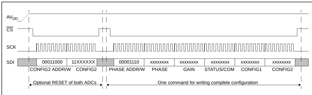
FIGURE 6-7: Recommended Configuration Sequence at Power Up.
