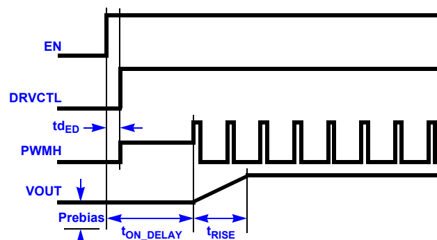
FIGURE 13. TURN-ON INTO PRE-BIAS
