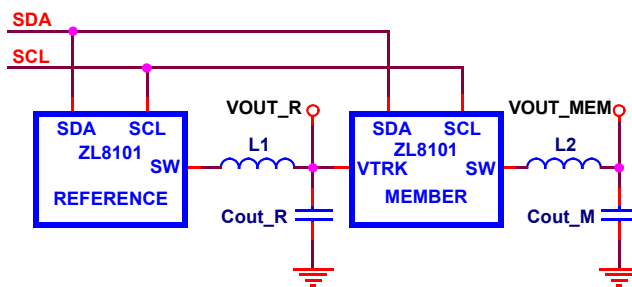
FIGURE 17. PMBus TRACKING
