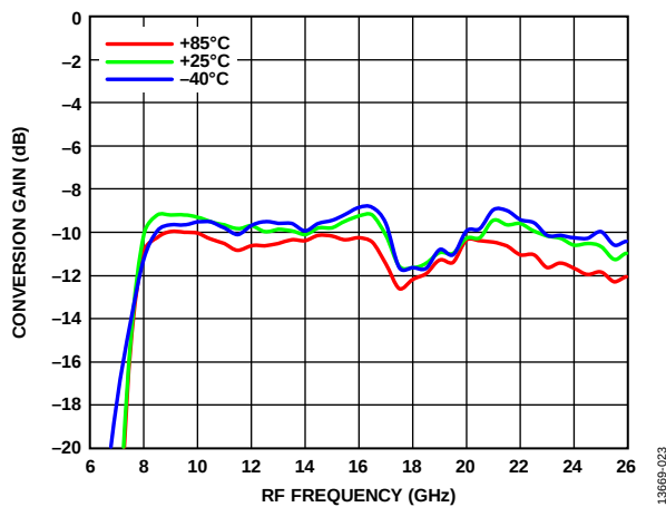
Figure 23. Conversion Gain vs. RF Frequency at Various Temperatures, LO Drive = 13 dBm
