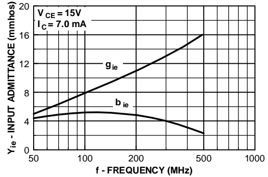
Input Admittance vs Frequency
