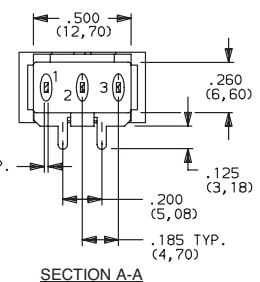
PC MOUNTING
