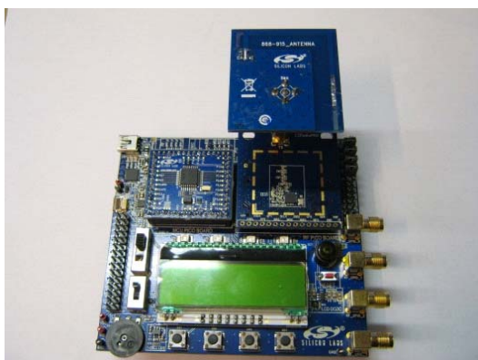
Figure 4. Medium Size Printed ILA
