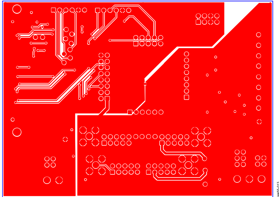
Figure 13. Motherboard Bottom Side Routing
