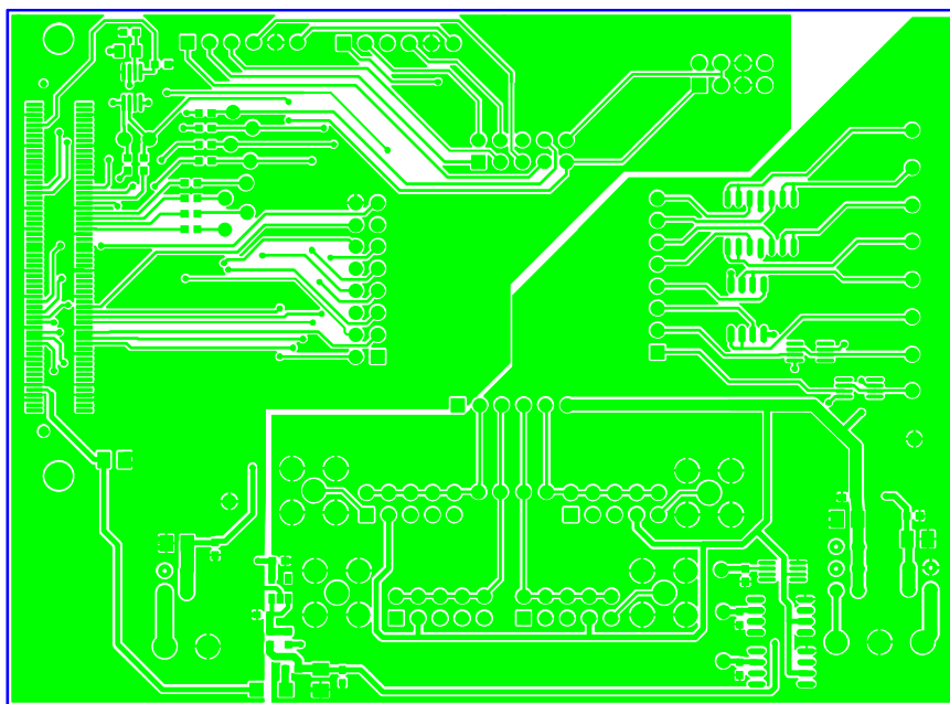
Figure 12. Motherboard Top Side Routing
