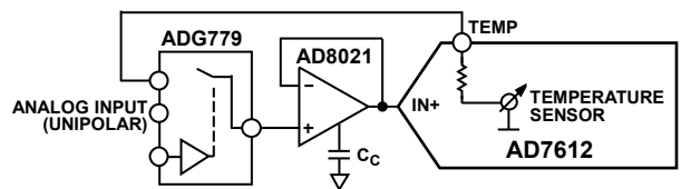
Figure 30. Use of the Temperature Sensor
