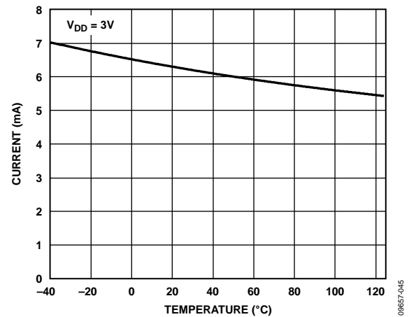
Figure 31. Maximum \overline{ASE} Output Current vs. Temperature
