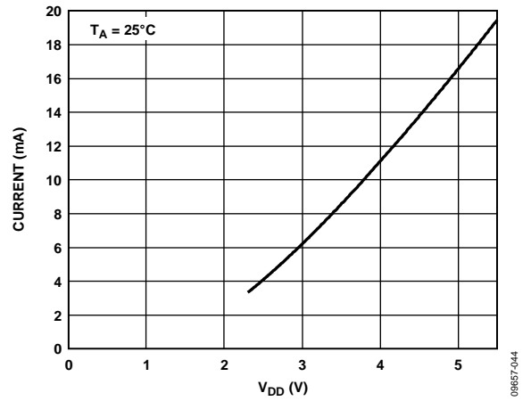
Figure 30. Maximum \overline{ASE} Output Current vs. Voltage
