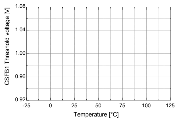
Figure 18. CS/FB Threshold Voltage vs. Temp.
