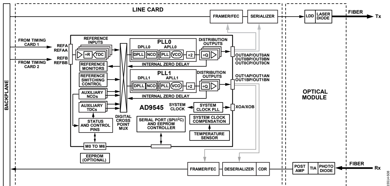
Figure 116. Optical Line Card Direct Timing Example
