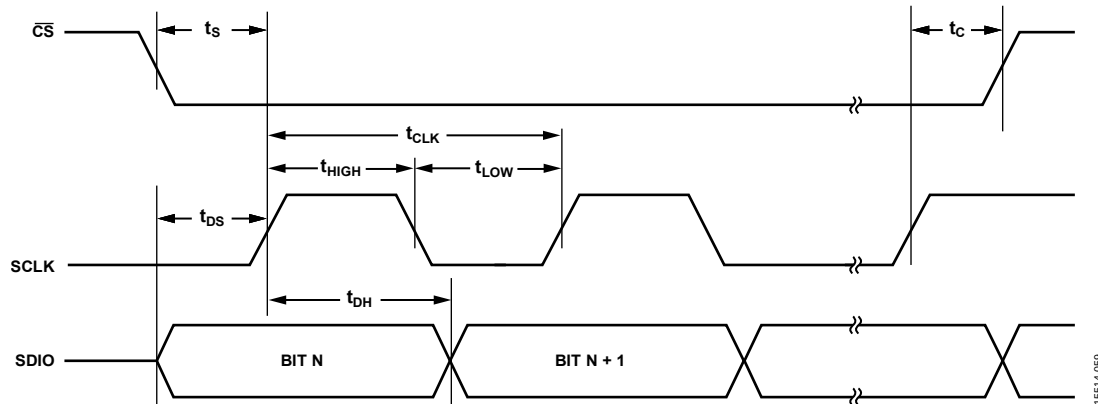
Figure 128. Serial Control Port Timing—Write
