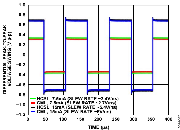
Figure 16. 8 kHz Output Waveforms for Various Driver Settings; HCSL Drivers Terminated 50\ \Omega to GND per Figure 38; CML Drivers Terminated 50\ \Omega to 1.8 V per Figure 39
