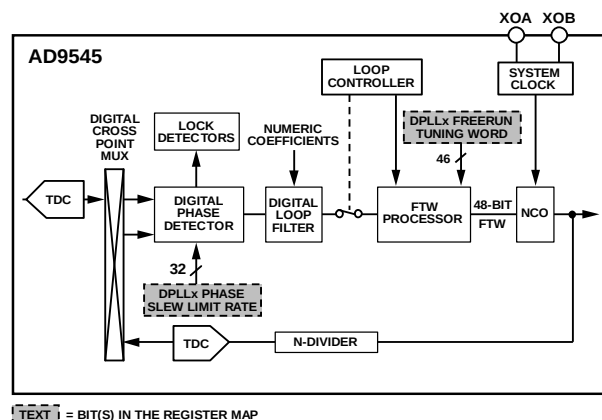
Figure 83. Phase Slew Limit Feature
