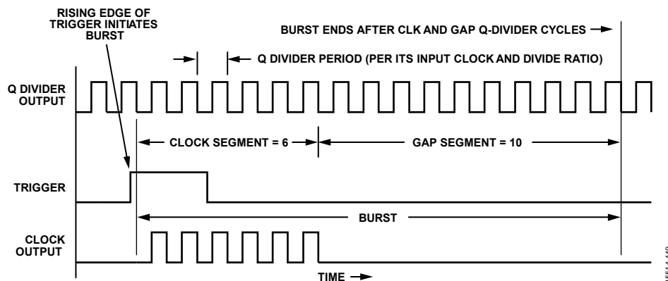
Figure 57. Burst Clock Signal
