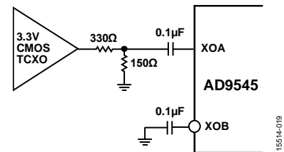
Figure 30. System Clock Input (XOA, XOB) When Using a TCXO/OCXO with 3.3 V CMOS Output
