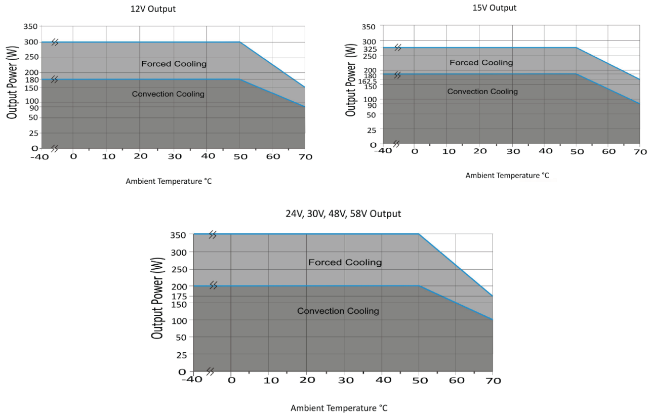
Figure 1. Derating Curves
