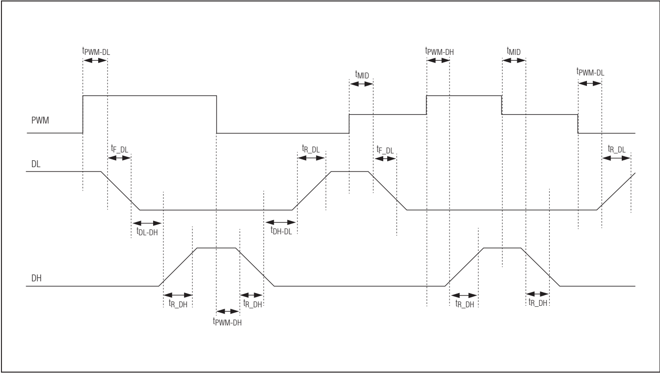
Figure 2. Timing Diagram
