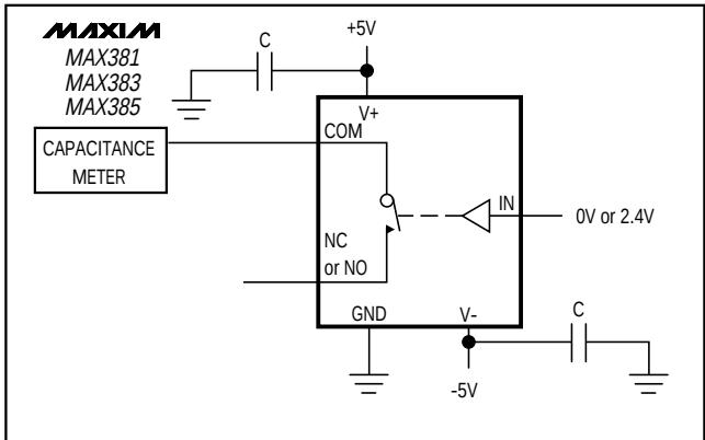
Figure 7. Channel-Off Capacitance
