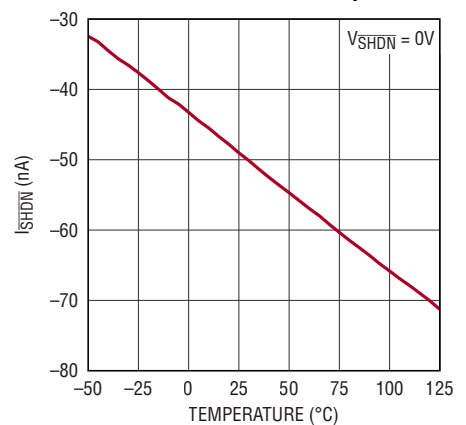
\overline{SHDN} Pin Current vs Temperature
