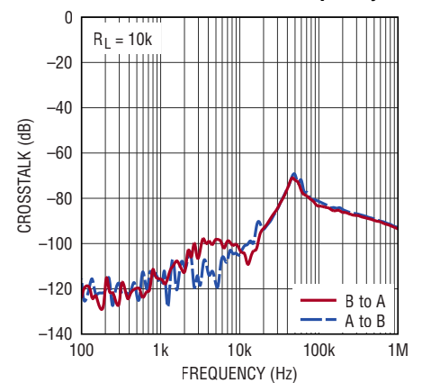
LTC2064 Crosstalk vs Frequency
