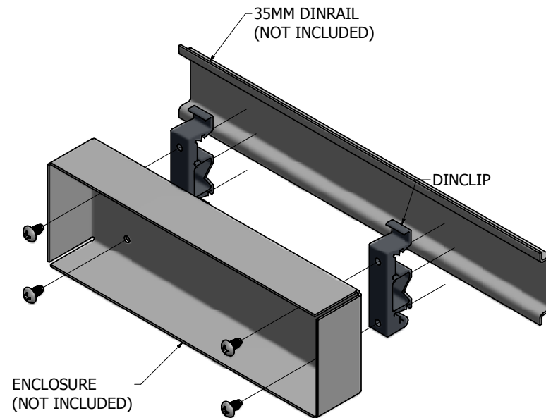
ISOMETRIC VIEW
