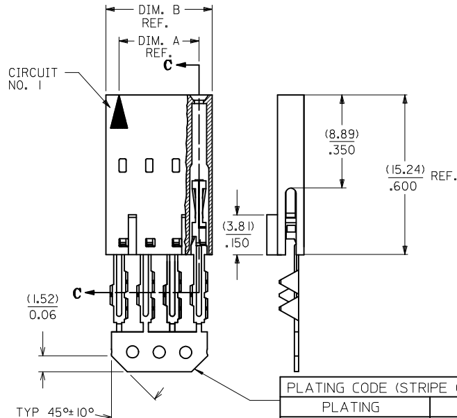
SECTION C-C
