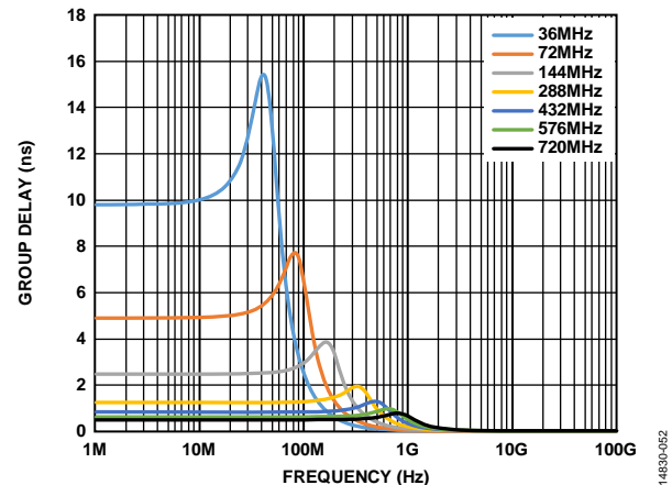
Figure 67. Ideal Fourth-Order Butterworth Group Delay Response for All 1 dB Bandwidths Programmed
