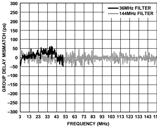
Figure 16. IQ Group Delay Mismatch vs. Frequency for 36 MHz and 144 MHz
