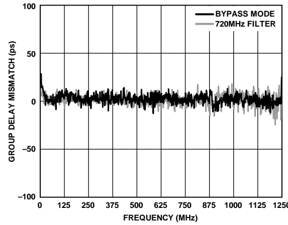
Figure 19. IQ Group Delay Mismatch vs. Frequency for 720 MHz and Bypass Mode
