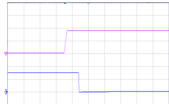
Figure 9 Output voltage shutdown by remote OFF, (20ms/div), see Figure 11 for test configuration; CH1-output voltage (1V/div); CH2-remote OFF voltage (2V/div) (Negative logic)
