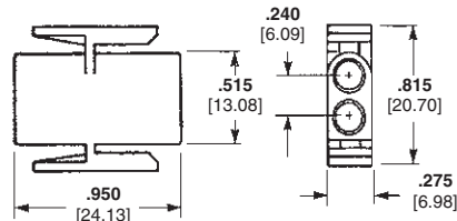
Socket Housing (Plug) Part No. 1-350344-0 Part No. 794699-1 (Black Color High Temp.)
