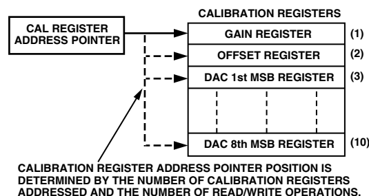
Figure 7. Calibration Register Arrangement
