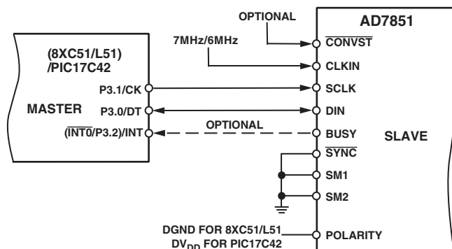
Figure 45. 8XC51/PIC17C42 Interface
