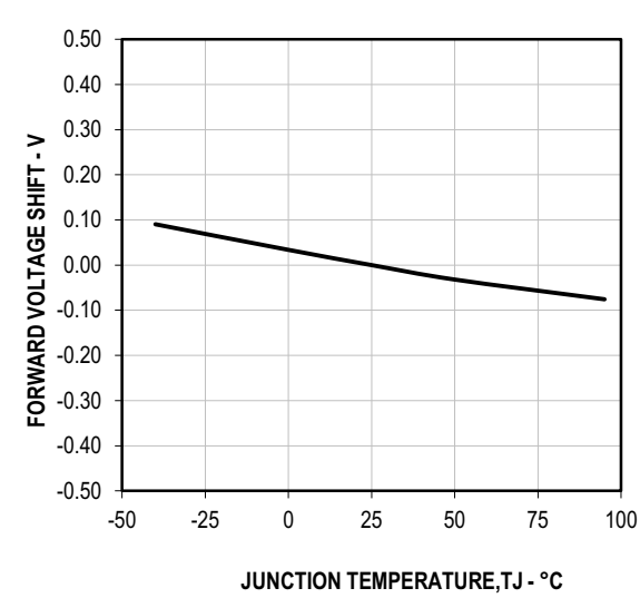
Figure 9: Forward Voltage vs. Temperature
