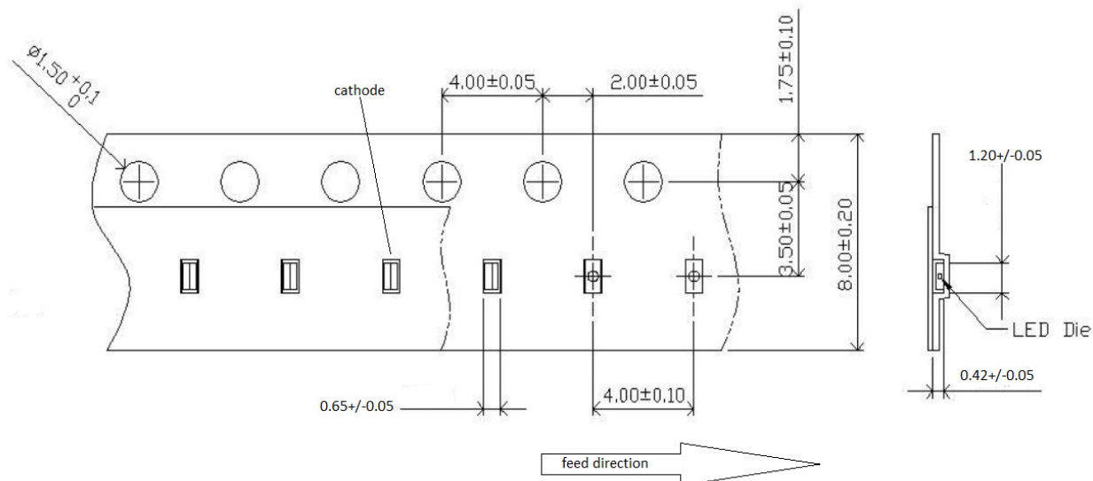
Figure 13: Carrier Tape Dimensions (Units: mm)
