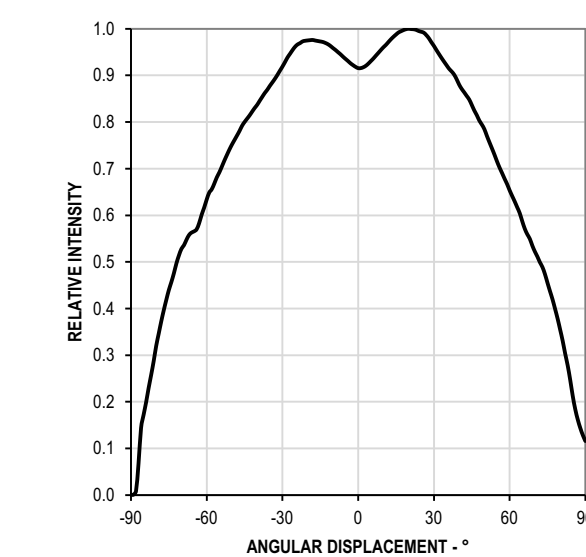
Figure 5: Intensity vs. Angle
