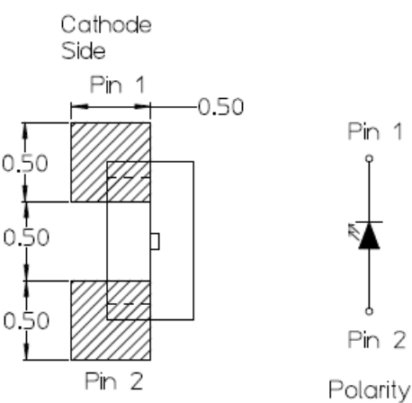
Figure 11: Recommended Solder Pad (Units: mm)
