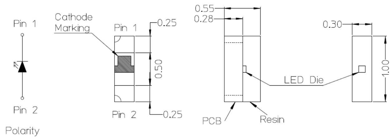
Figure 1: Package Dimensions
