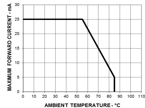
Figure 10: Forward Current vs. Temperature
