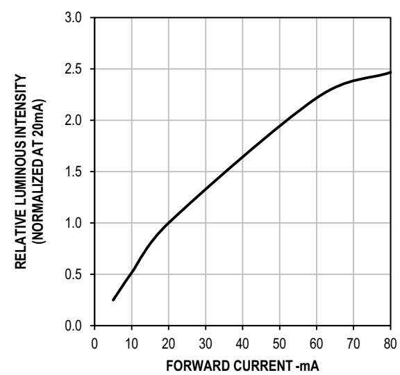
Figure 4: Intensity vs. Forward Current
