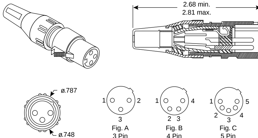
Dimensions (In.)
