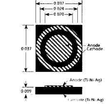
Figure 2 Chip
