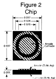
Figure 2 Chip Anode (Ti-Ni-Ag) Cathode (Ti-Ni-Ag) Metallization Substrate Dimensions: Nominal (Inches)
