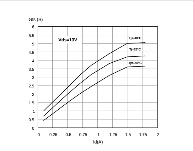
Figure 14. Transconductance
