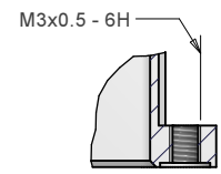
HARDWARE OPTION M3-0 (THREADED HOLES M3)
