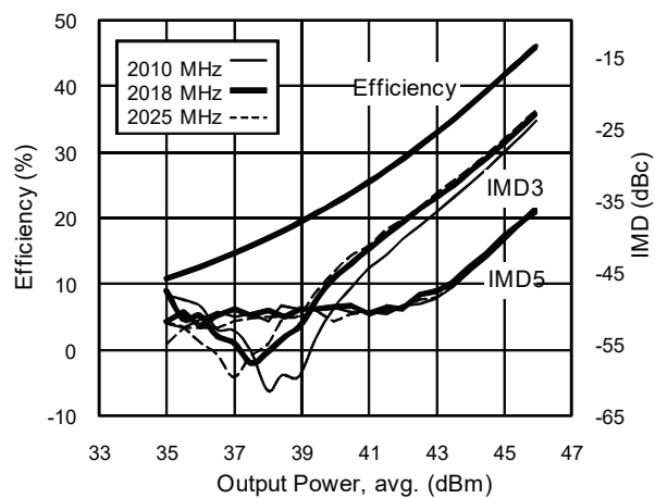
Two-tone Performance at Selected Frequencies single side, V_{DD} = 28 \text{ V} , I_{DQ} = 650 \text{ mA} , 1 MHz tone spacing
