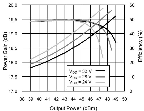
CW Gain & Eff. vs. Output Power at various V_{DD} , single side I_{DQ} = 650 \text{ mA} , f = 2018 \text{ MHz}
