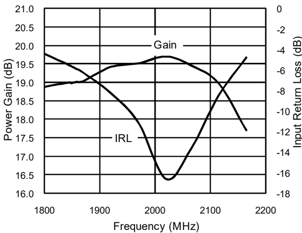
Small Signal CW Gain & Input Return Loss, single side V_{DD} = 28\text{ V} , I_{DQ} = 650\text{ mA}
