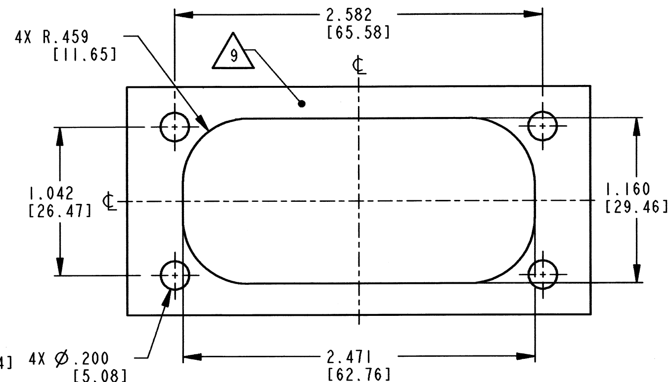
PANEL CUTOUT
