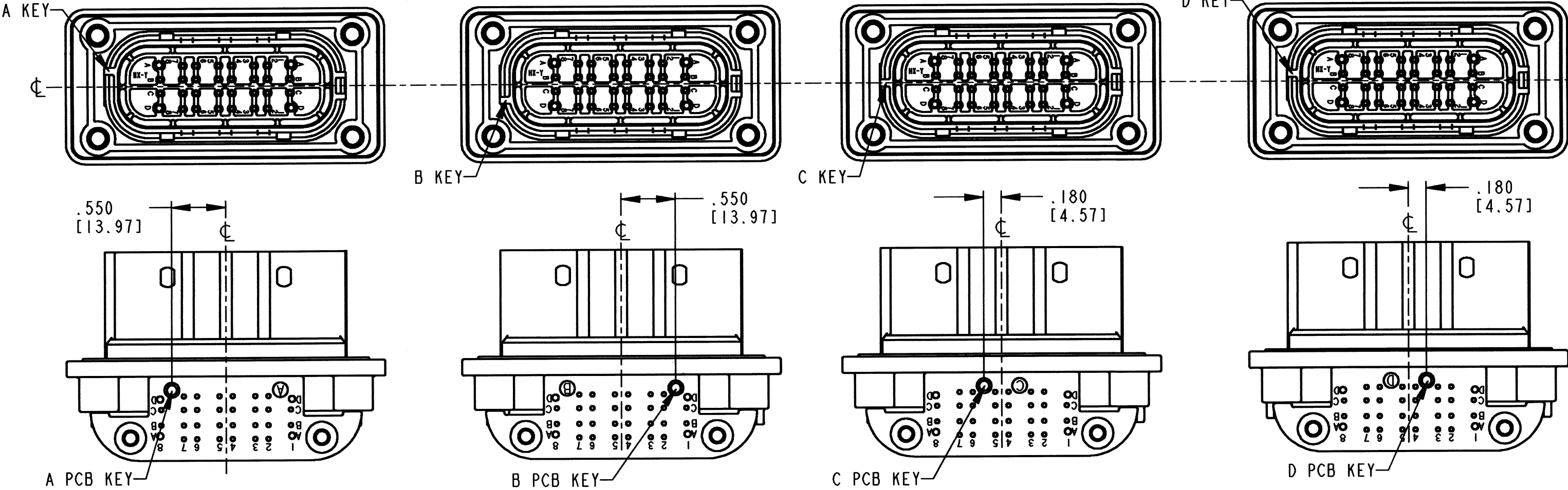
KEY ARRANGEMENT -D- SRK13-MDD-32A-001
