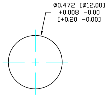
PANEL CUTOUT
