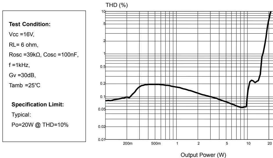
Figure 20. THD vs. output power (1 kHz)
