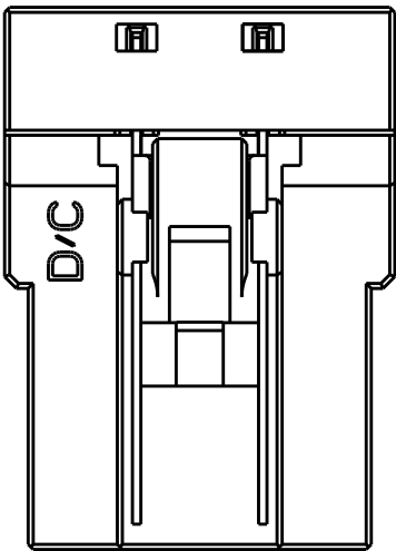
3POS(Y-KEY): 4-2013522-3
