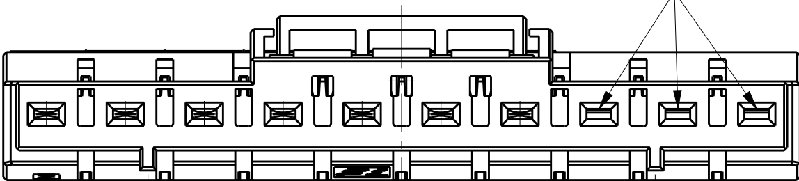
7/10POS(Z-KEY) CIRCUIT 1~7:9-2013522-0
