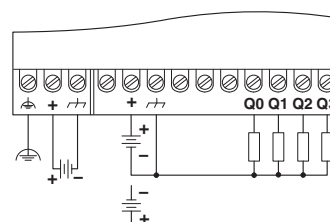
Connection diagram
