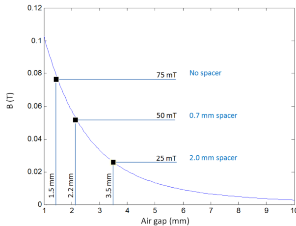
Figure 14: Magnetic Field vs. Air Gap for the Supplied Magnet
