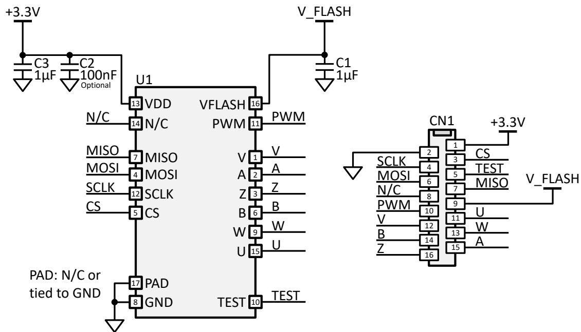
Figure 4: Schematic Type 1
