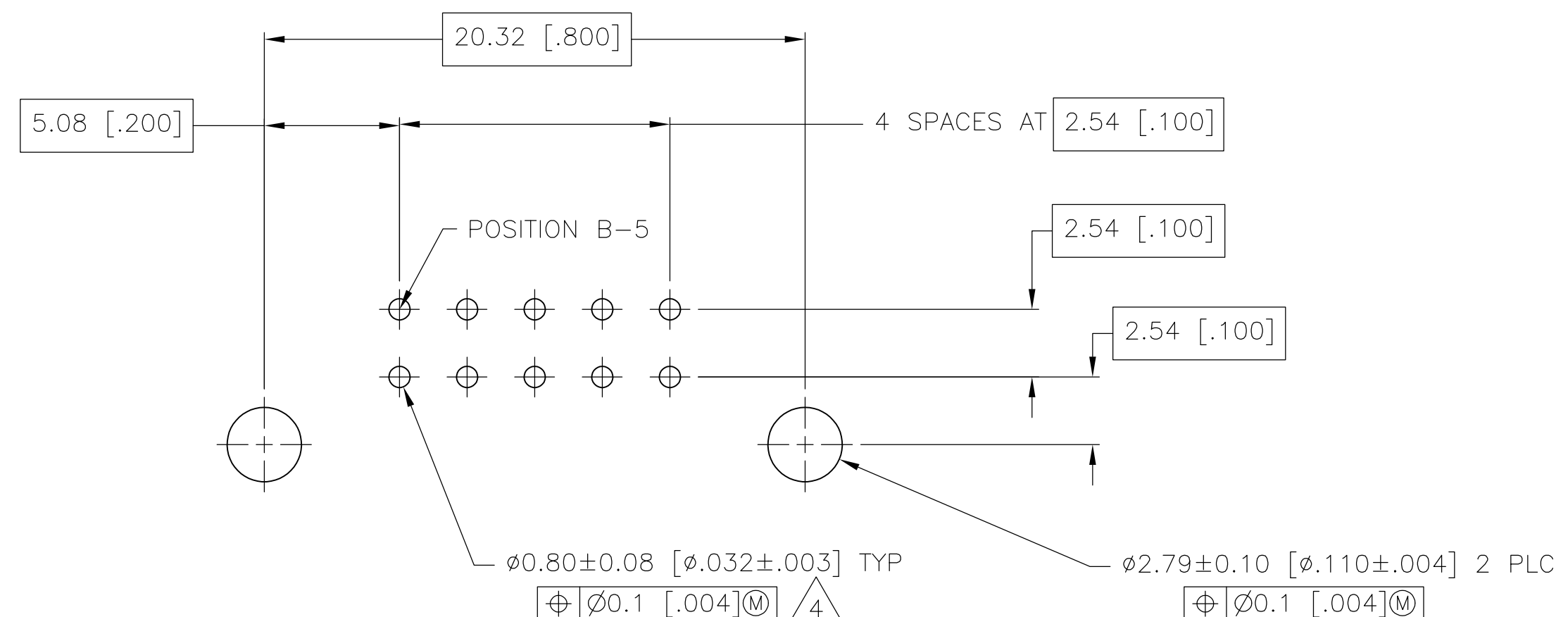
PC BOARD LAYOUT
