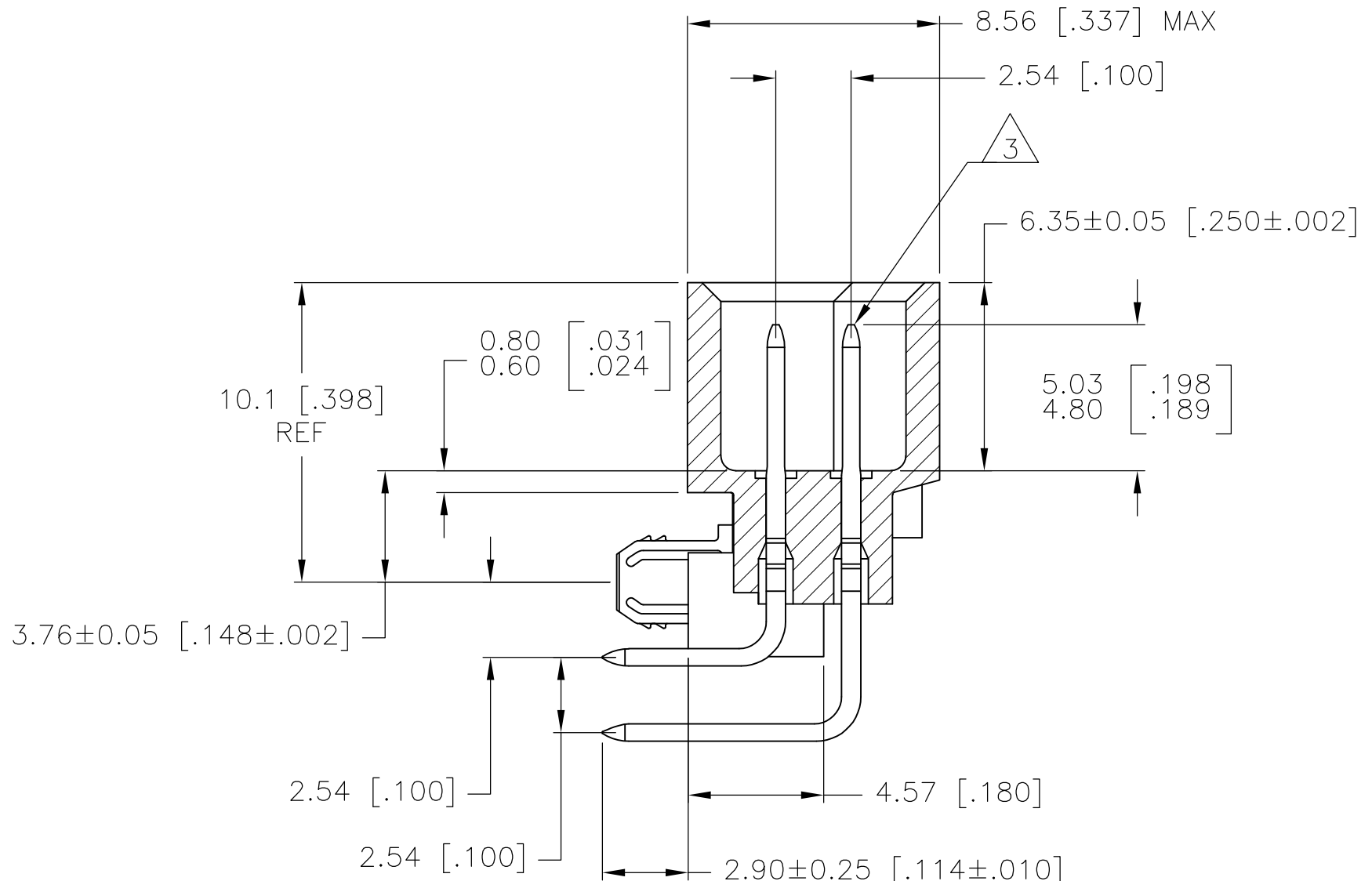
SECTION Z-Z
